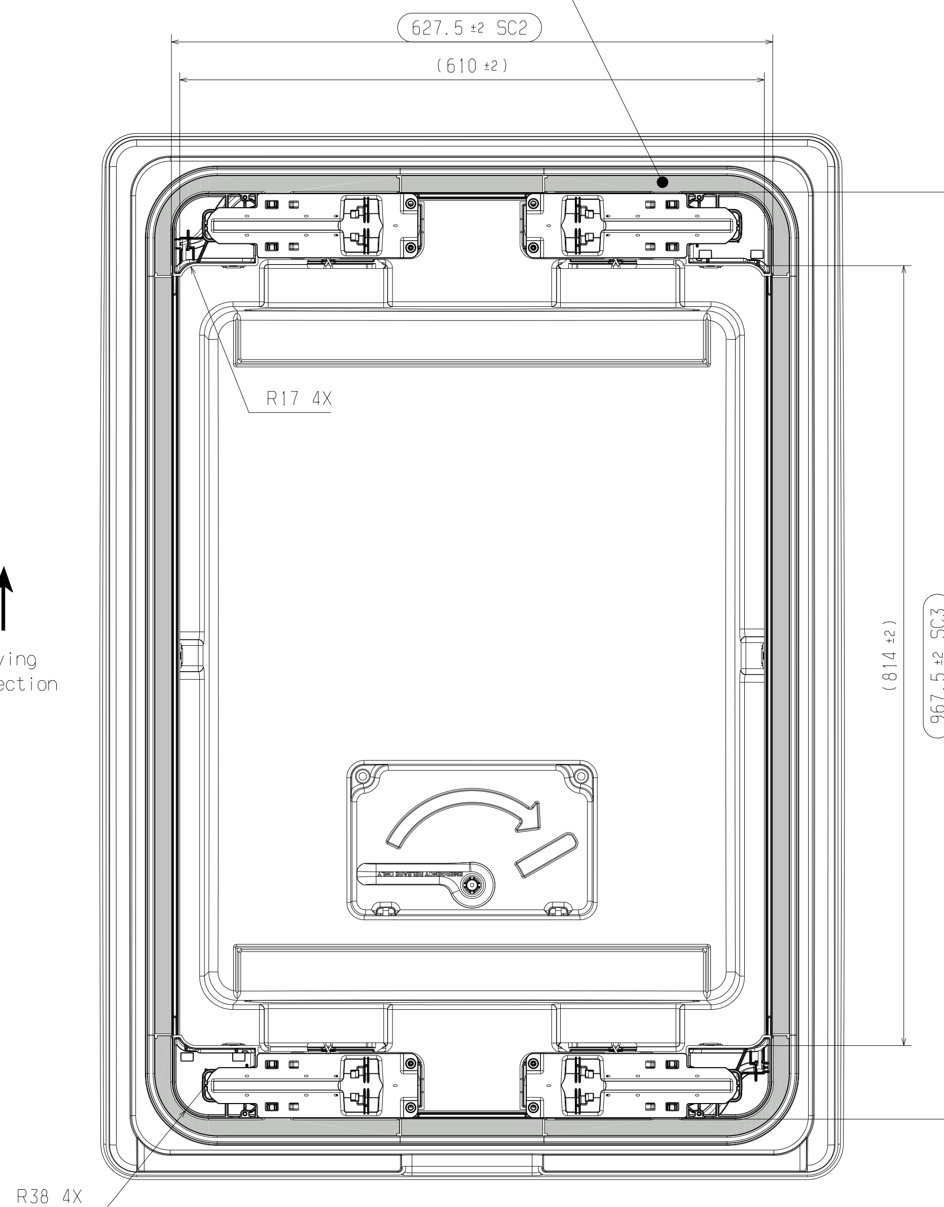
Bottom view, no inner frame, no inner emergency handle cover Scale: 1:4
