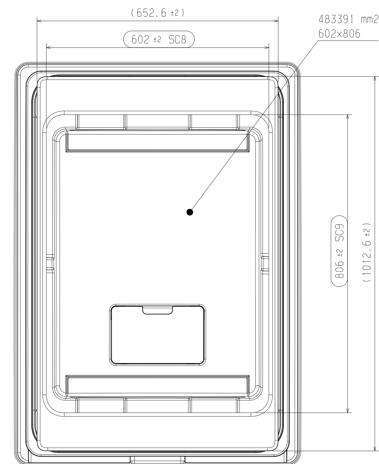
Bottom view with inner frame Scale: 1:6
